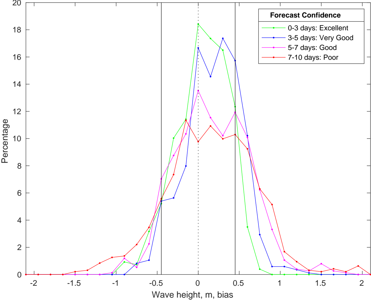
NDBC 46011 vs CMEMS Waves Bias Histogram: 01-Jun-2025
