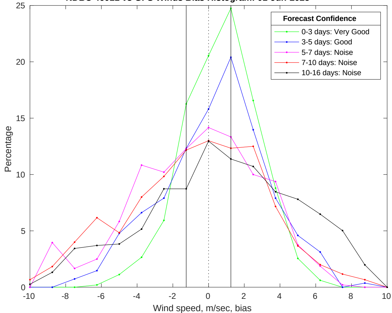
NDBC 46011 vs GFS Winds Bias Histogram: 01-Jun-2025
