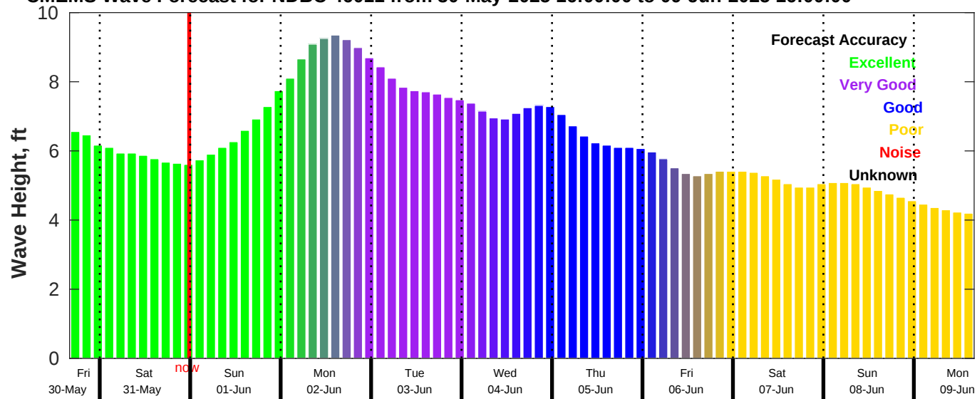
CMEMS Wave Forecast for NDBC 46011 from 30-May-2025 16:00:00 to 09-Jun-2025 16:00:00
