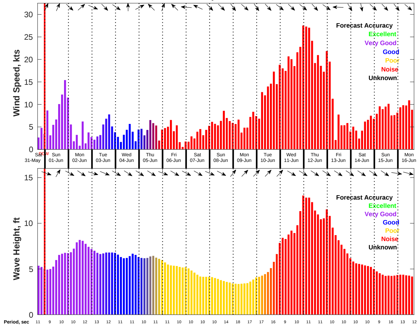
Wind & Wave Forecast for NDBC 46011 from 31-May-2025 16:00:00 to 16-Jun-2025 16:00:00
