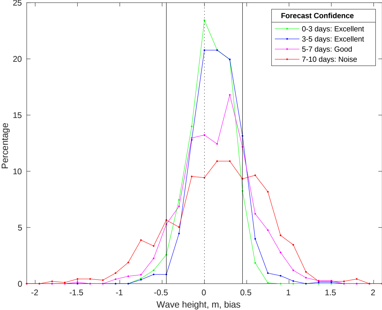
NDBC 46028 vs CMEMS Waves Bias Histogram: 01-Jun-2025
