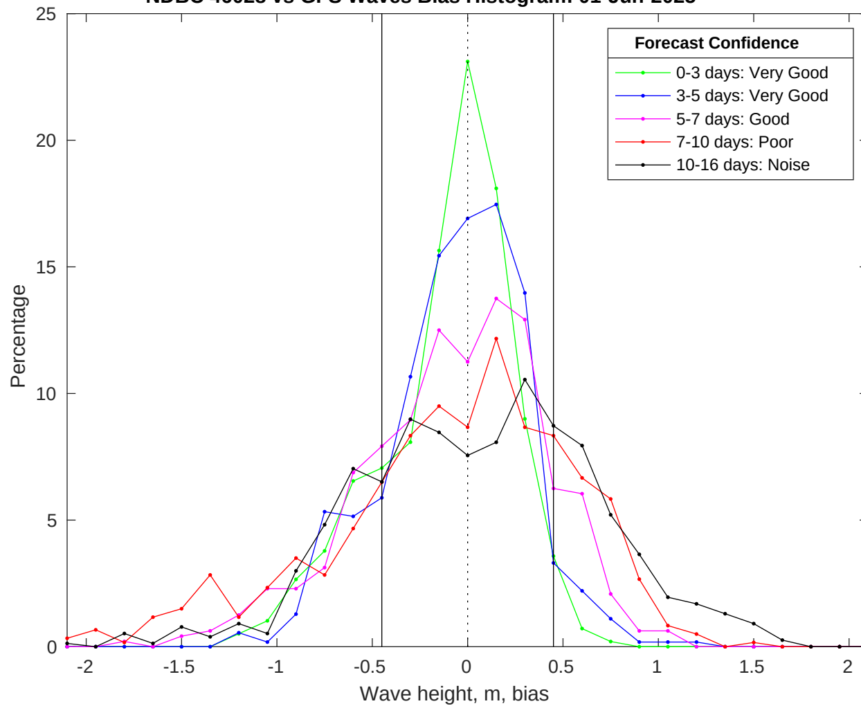
NDBC 46028 vs GFS Waves Bias Histogram: 01-Jun-2025
