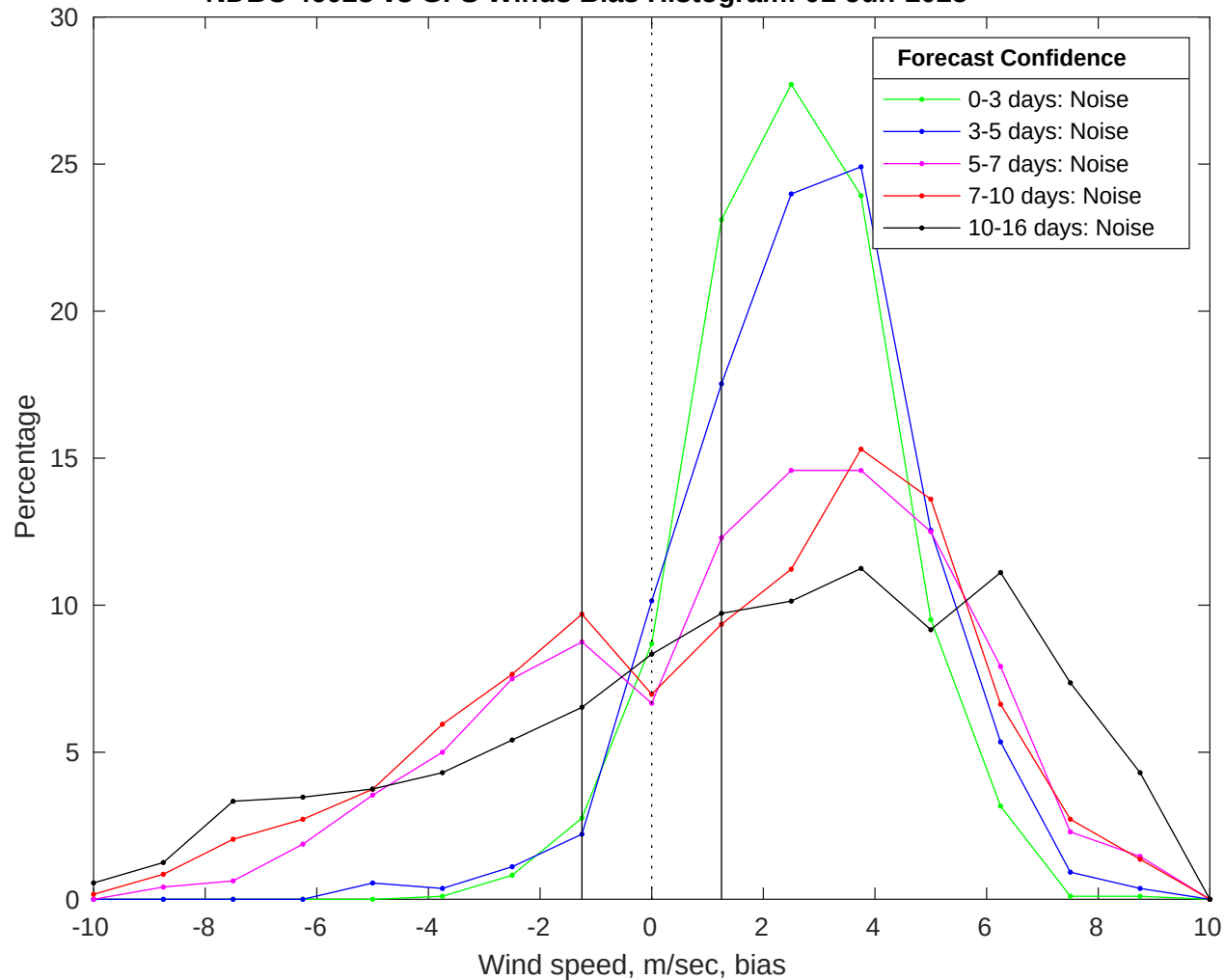
NDBC 46028 vs GFS Winds Bias Histogram: 01-Jun-2025
