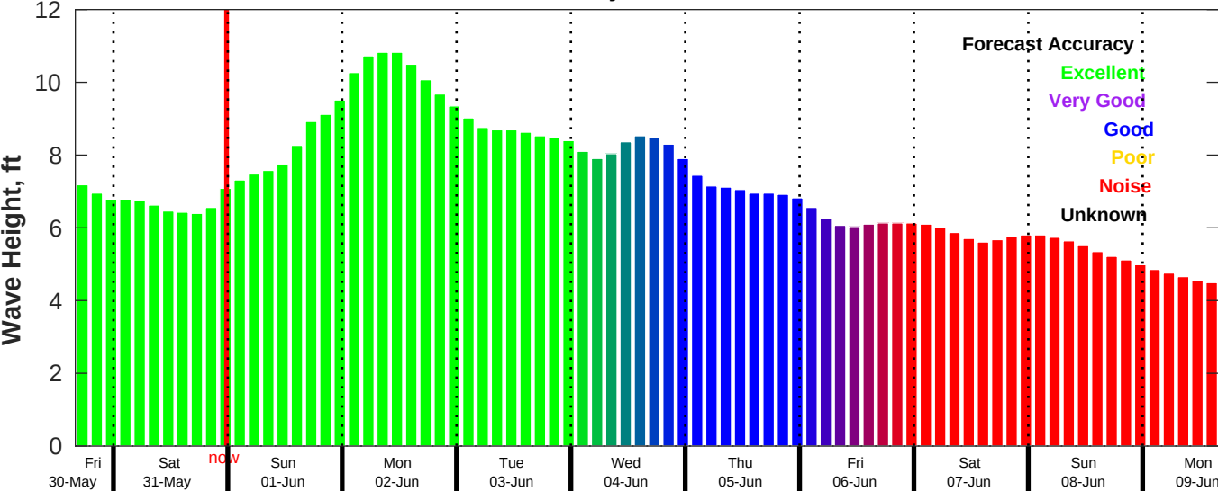
CMEMS Wave Forecast for NDBC 46028 from 30-May-2025 16:00:00 to 09-Jun-2025 16:00:00
