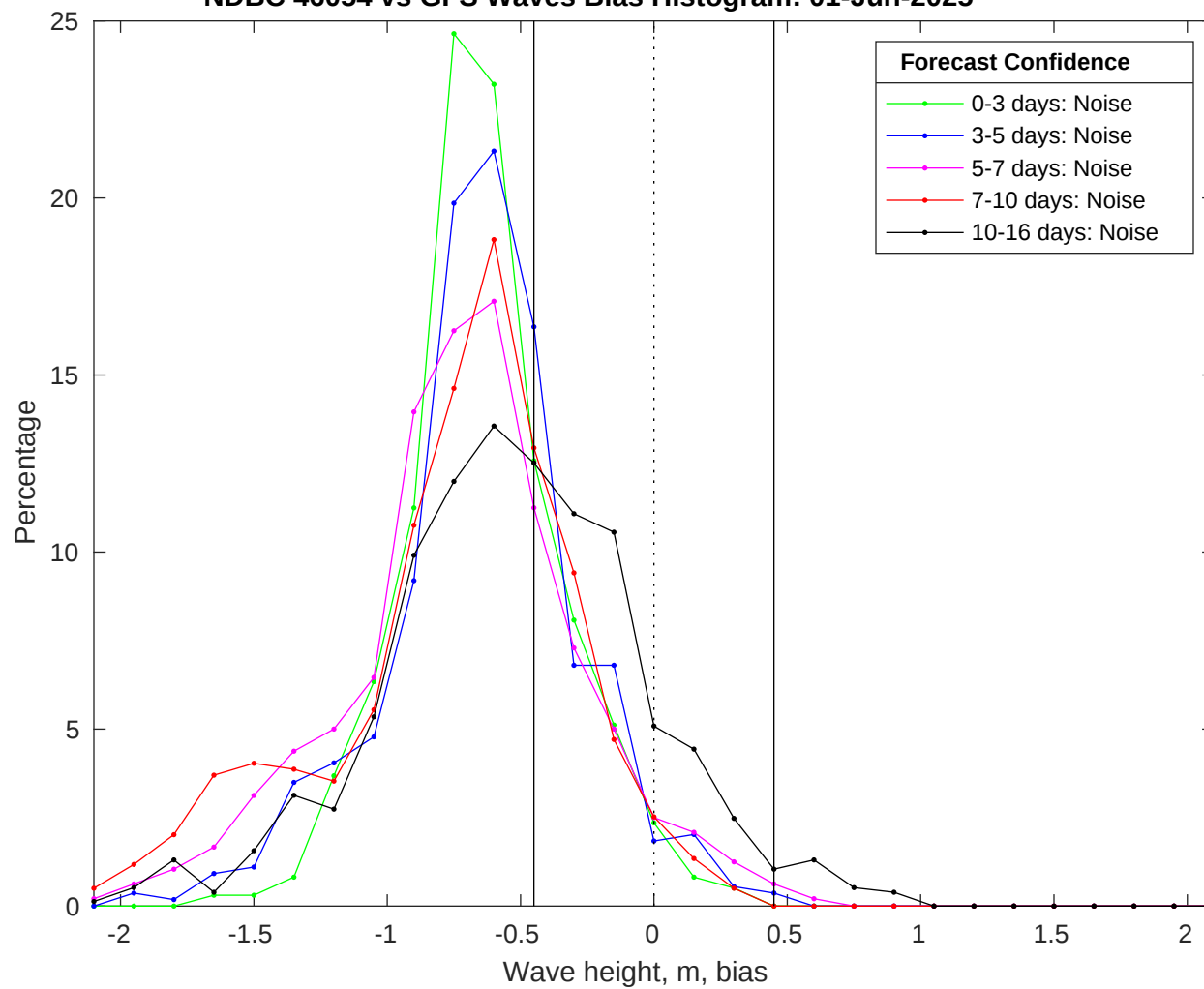
NDBC 46054 vs GFS Waves Bias Histogram: 01-Jun-2025
