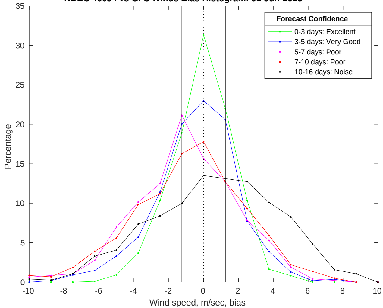
NDBC 46054 vs GFS Winds Bias Histogram: 01-Jun-2025
