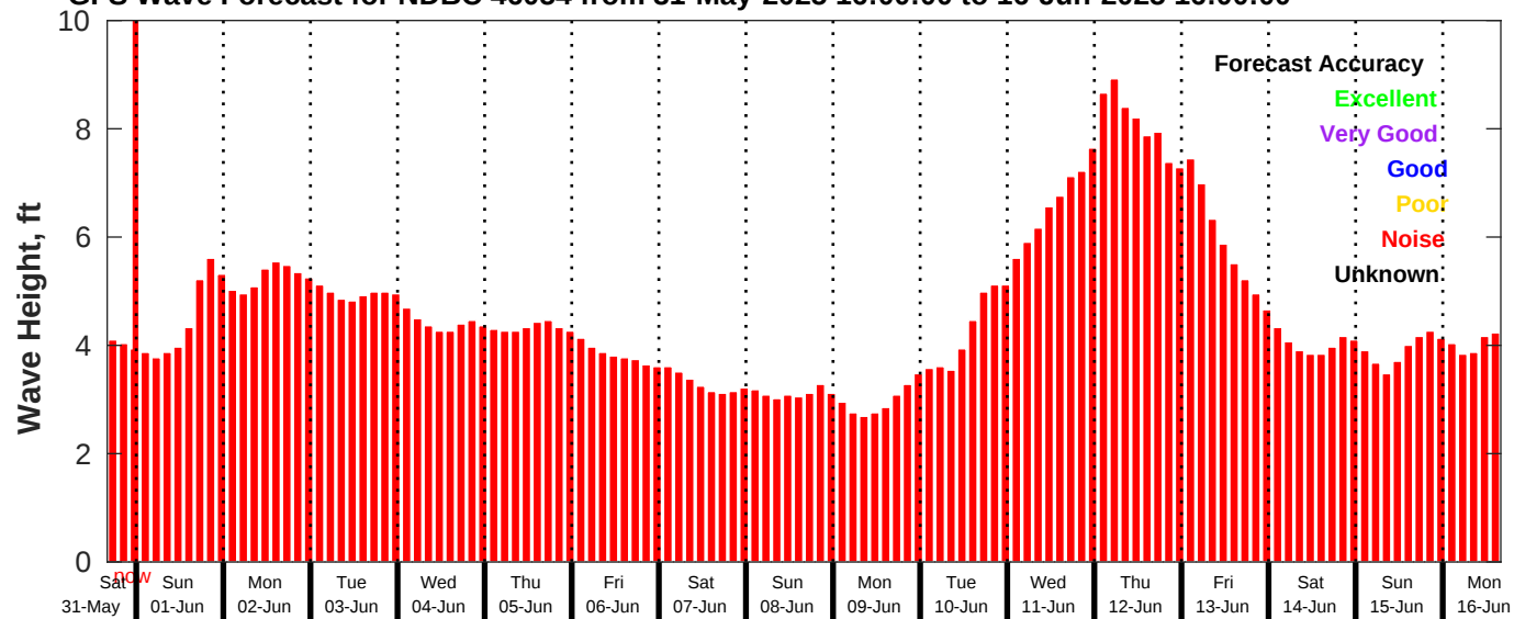
GFS Wave Forecast for NDBC 46054 from 31-May-2025 16:00:00 to 16-Jun-2025 16:00:00
