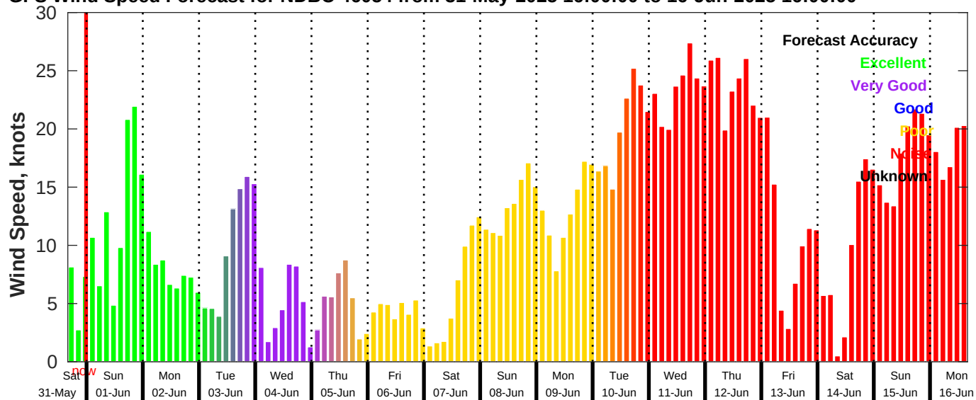
GFS Wind Speed Forecast for NDBC 46054 from 31-May-2025 16:00:00 to 16-Jun-2025 16:00:00
