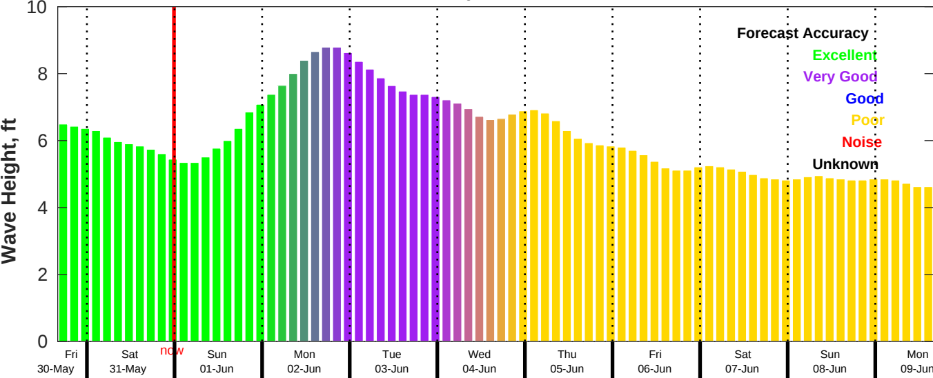
CMEMS Wave Forecast for NDBC 46069 from 30-May-2025 16:00:00 to 09-Jun-2025 16:00:00
