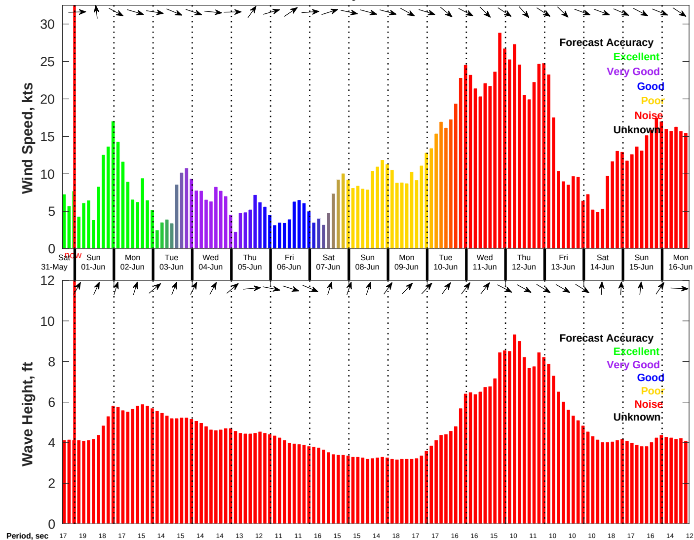
Wind & Wave Forecast for NDBC 46069 from 31-May-2025 16:00:00 to 16-Jun-2025 16:00:00
