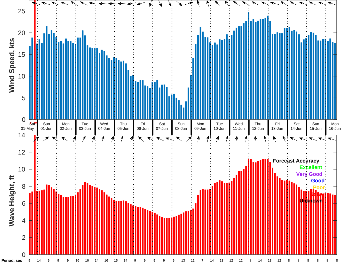
Wind & Wave Forecast for NDBC 51209 from 31-May-2025 13:00:00 to 16-Jun-2025 13:00:00
