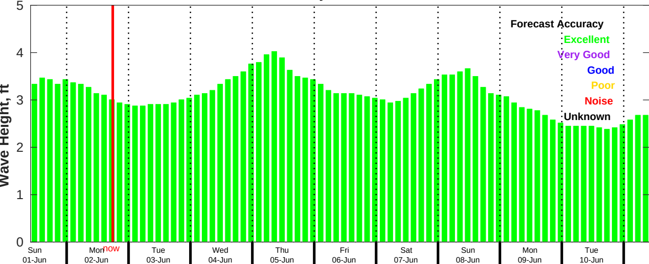
CMEMS Wave Forecast for NDBC 52211 from 31-May-2025 10:00:00 to 10-Jun-2025 10:00:00
