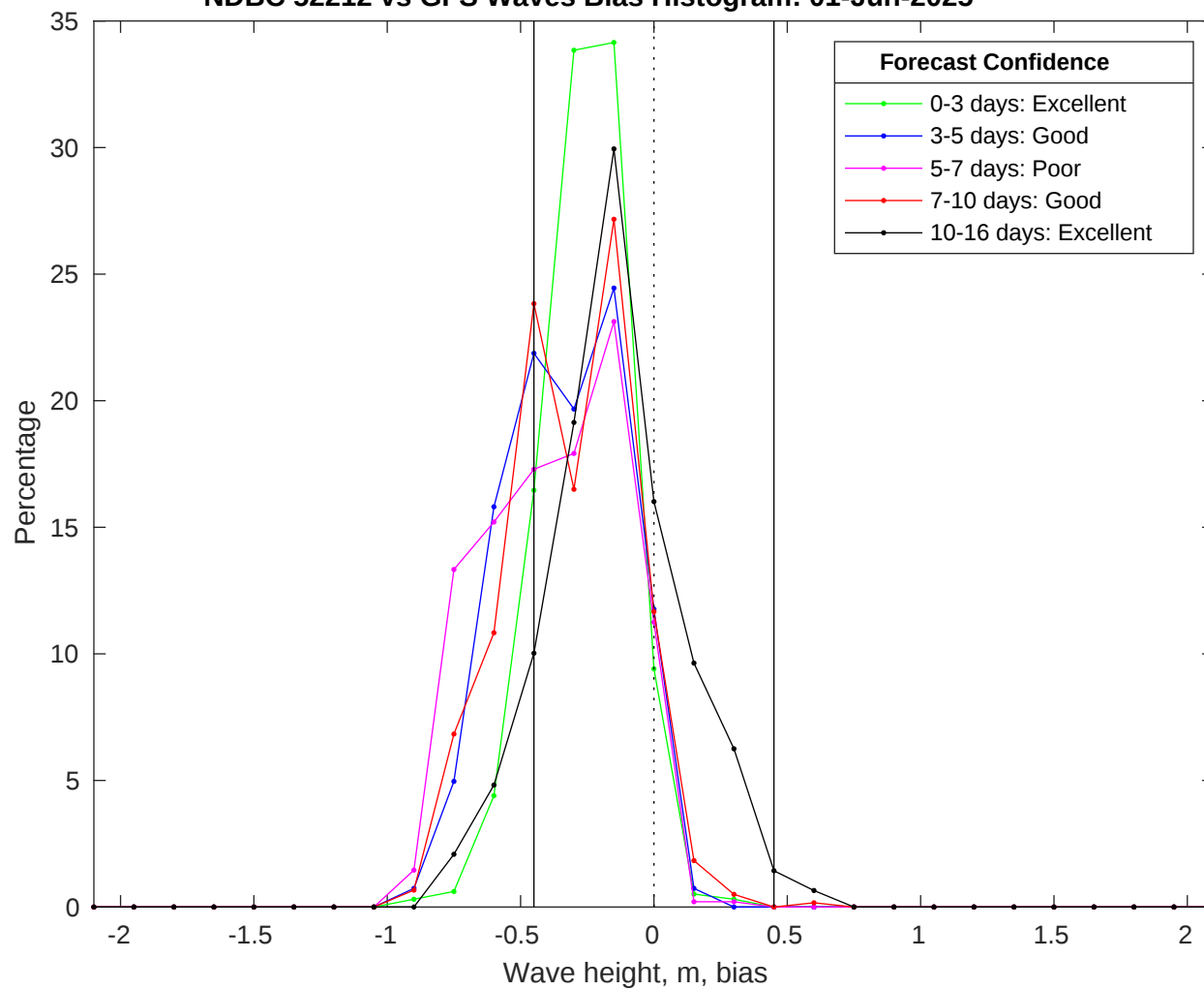
NDBC 52212 vs GFS Waves Bias Histogram: 01-Jun-2025
