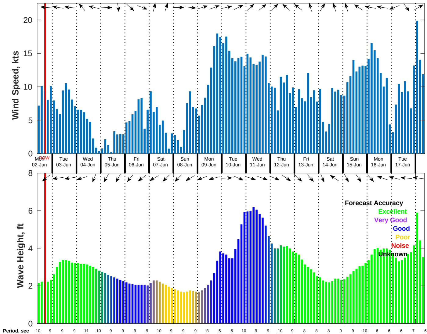
Wind & Wave Forecast for NDBC 52212 from 01-Jun-2025 09:00:00 to 17-Jun-2025 09:00:00
