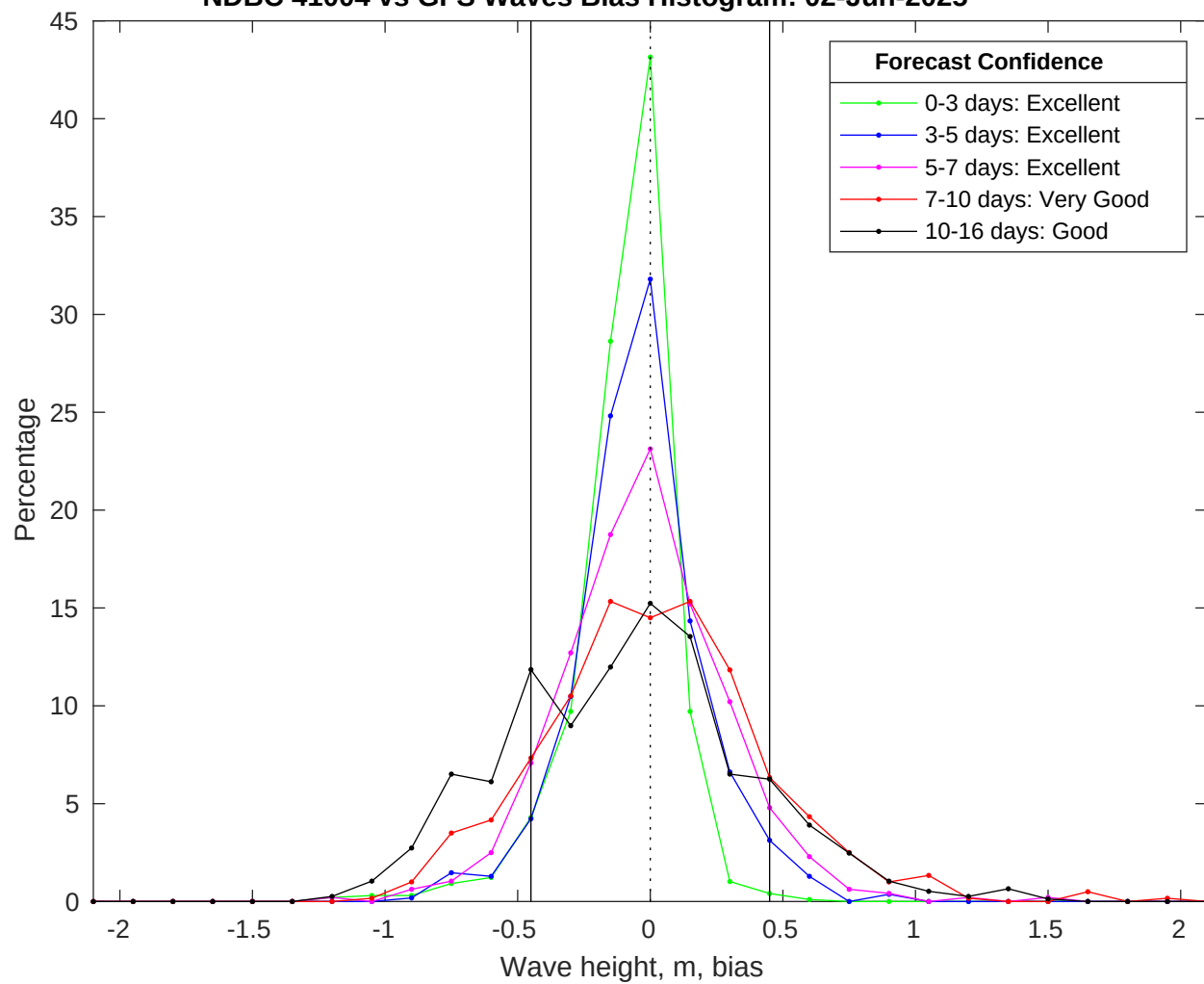
NDBC 41004 vs GFS Waves Bias Histogram: 02-Jun-2025
