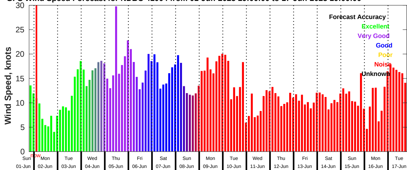
GFS Wind Speed Forecast for NDBC 41004 from 01-Jun-2025 19:00:00 to 17-Jun-2025 19:00:00
