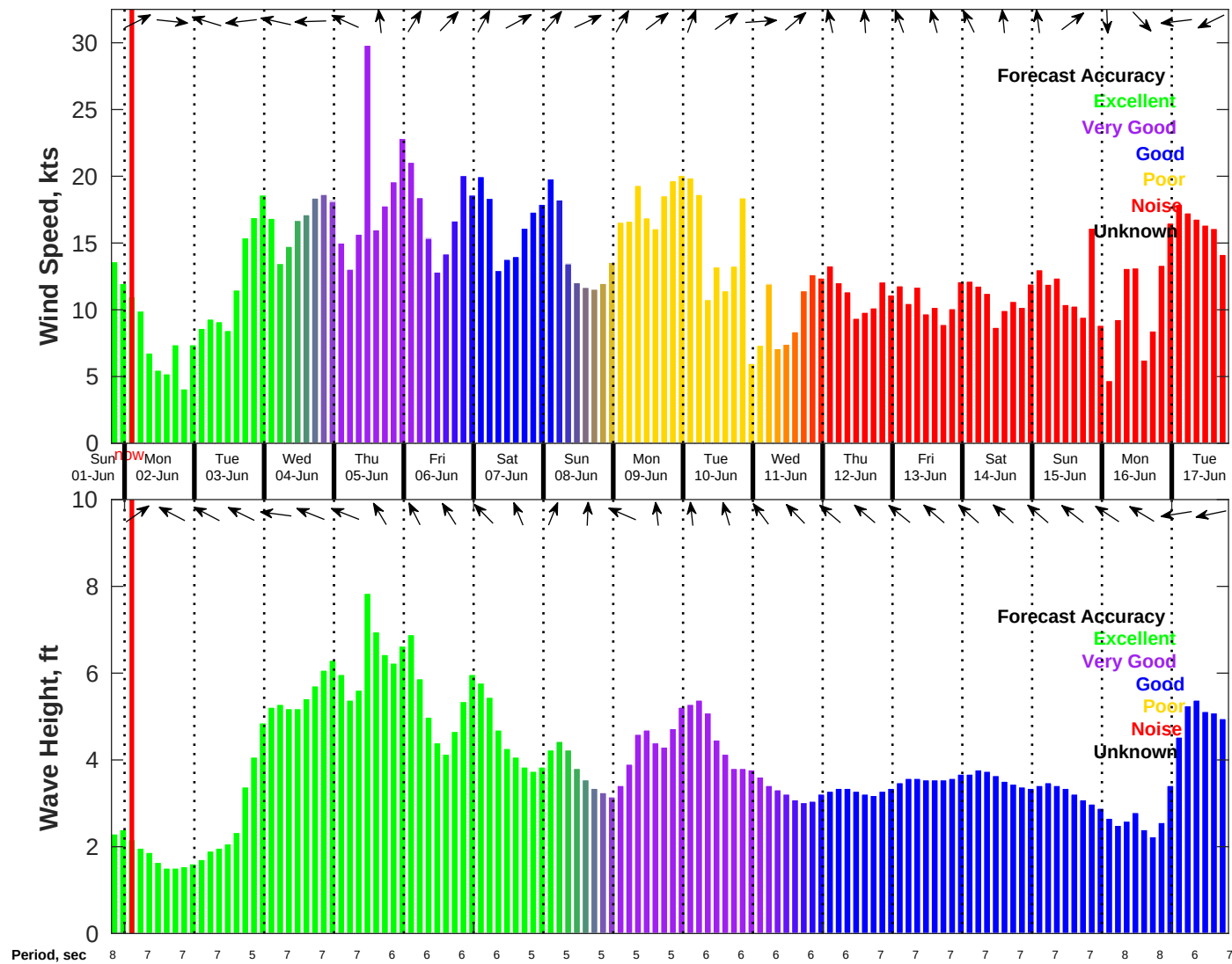
Wind & Wave Forecast for NDBC 41004 from 01-Jun-2025 19:00:00 to 17-Jun-2025 19:00:00
