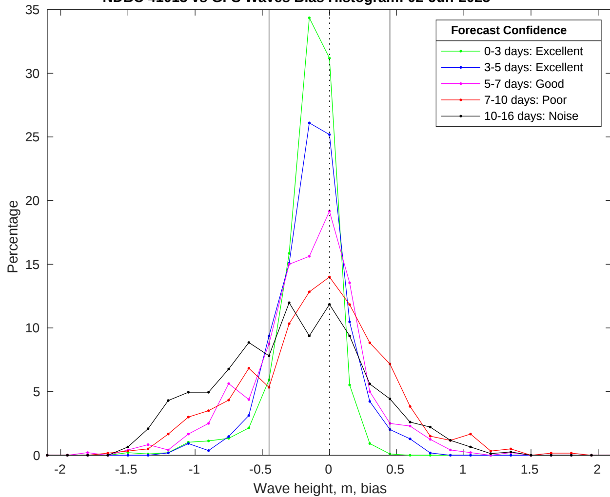
NDBC 41013 vs GFS Waves Bias Histogram: 02-Jun-2025
