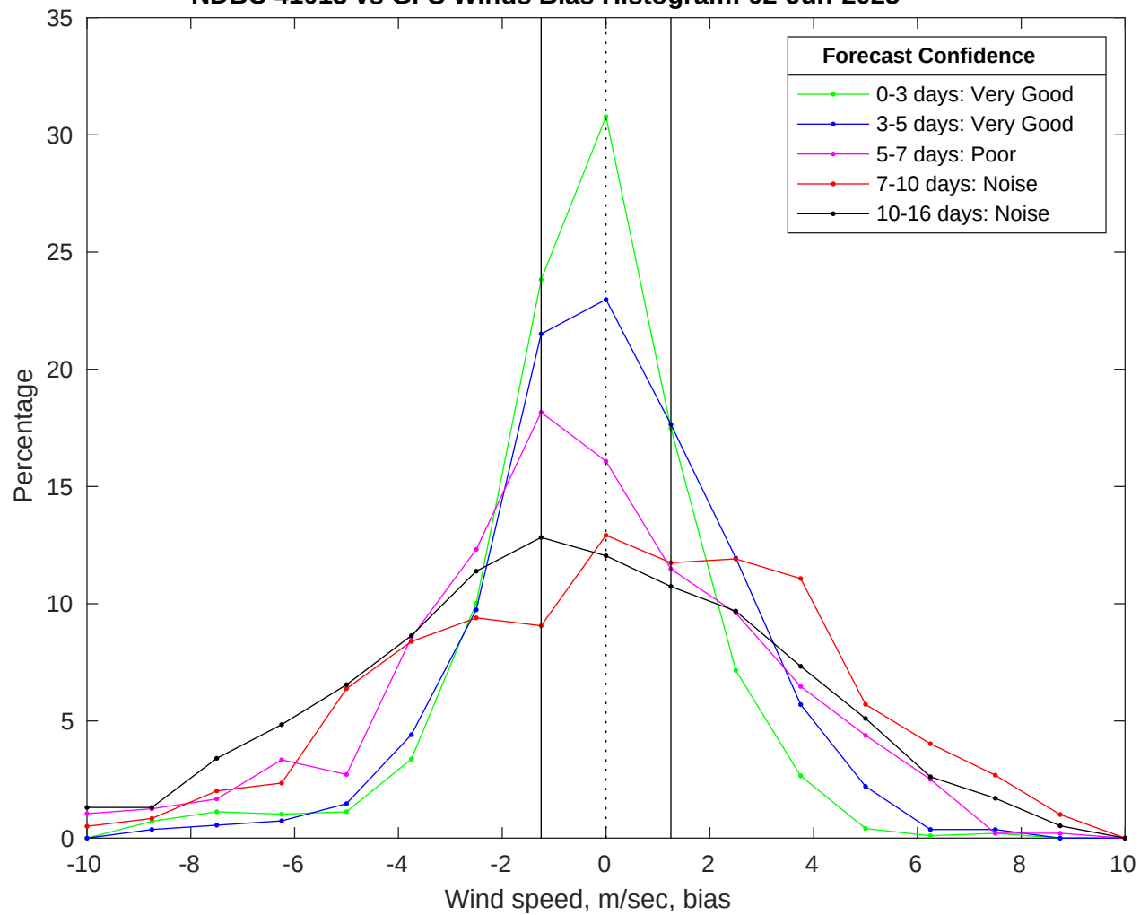
NDBC 41013 vs GFS Winds Bias Histogram: 02-Jun-2025
