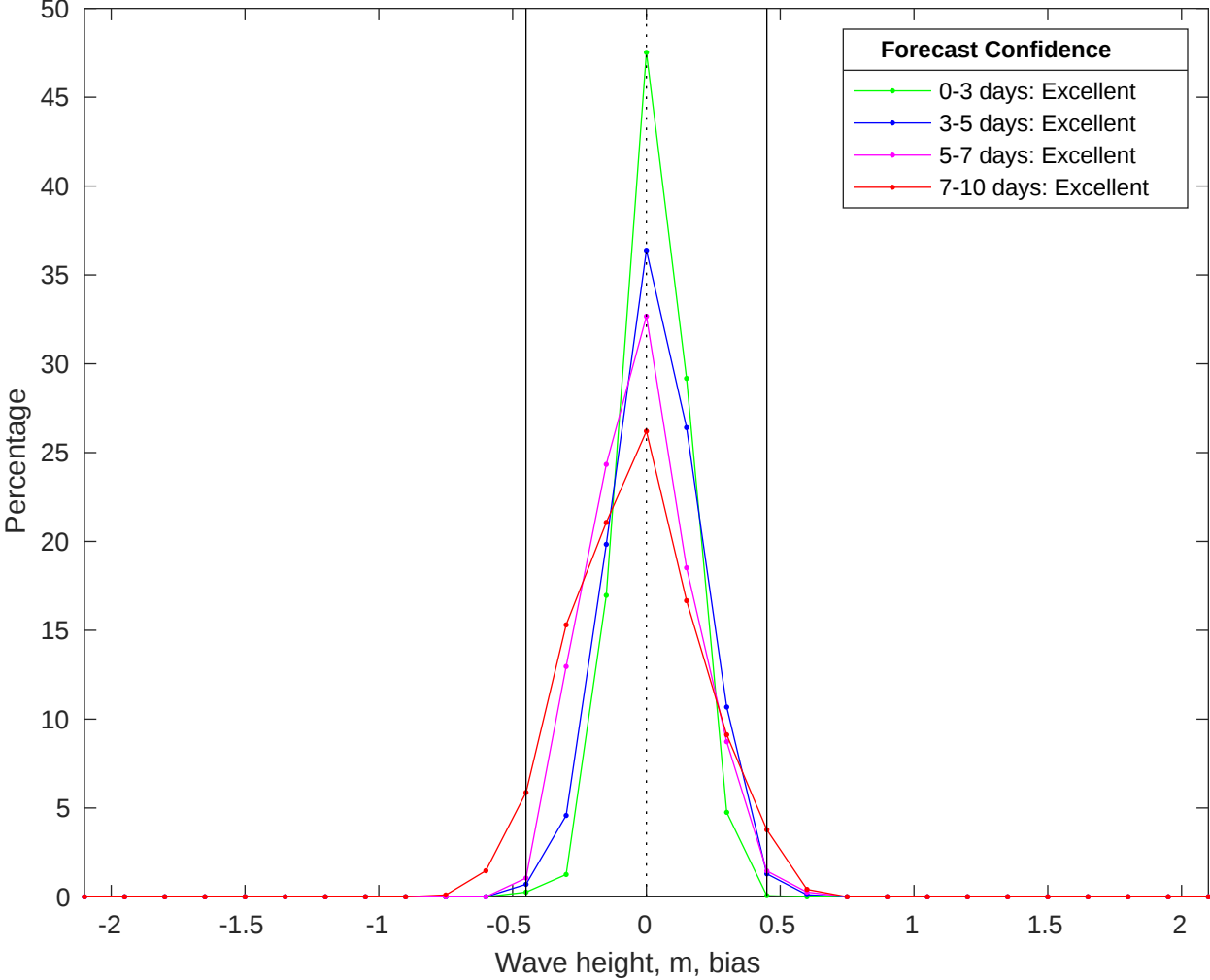
NDBC 41040 vs CMEMS Waves Bias Histogram: 02-Jun-2025
