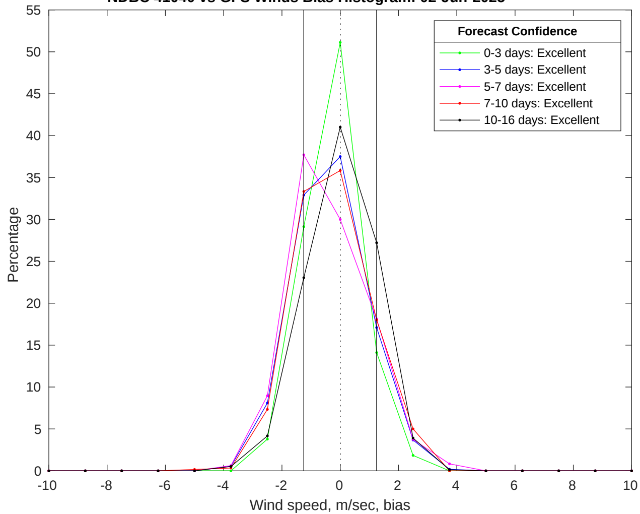
NDBC 41040 vs GFS Winds Bias Histogram: 02-Jun-2025
