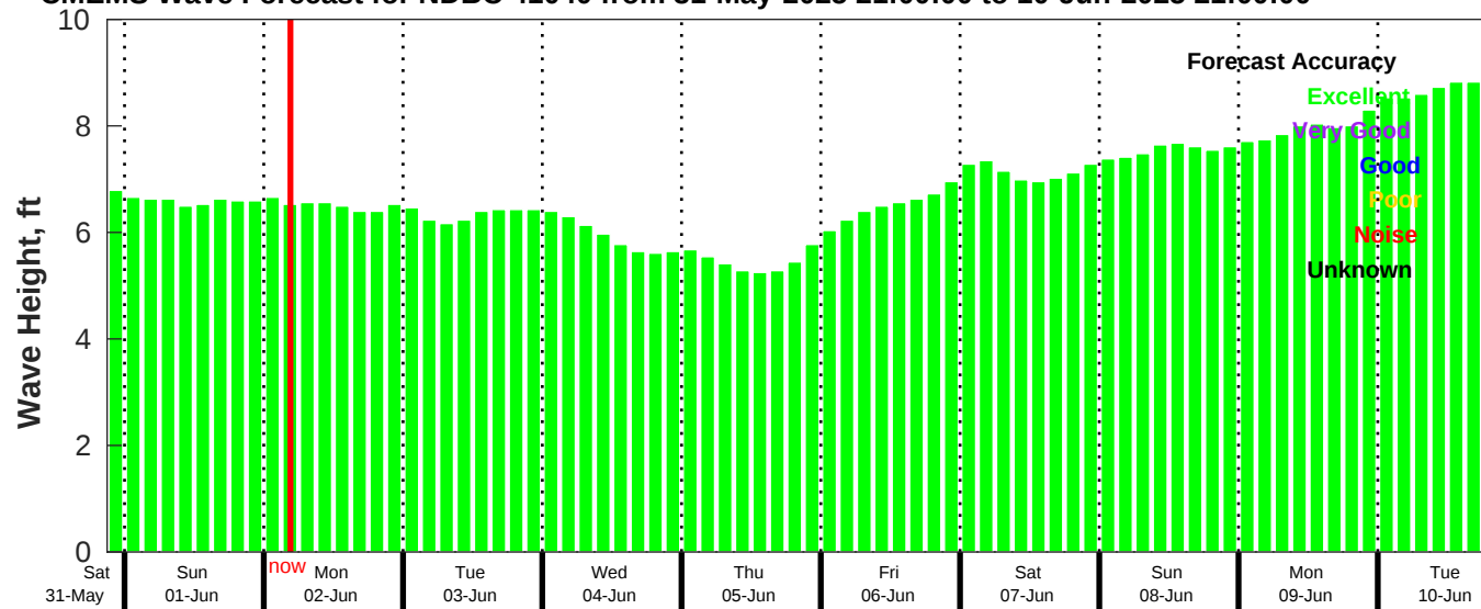
CMEMS Wave Forecast for NDBC 41040 from 31-May-2025 21:00:00 to 10-Jun-2025 21:00:00
