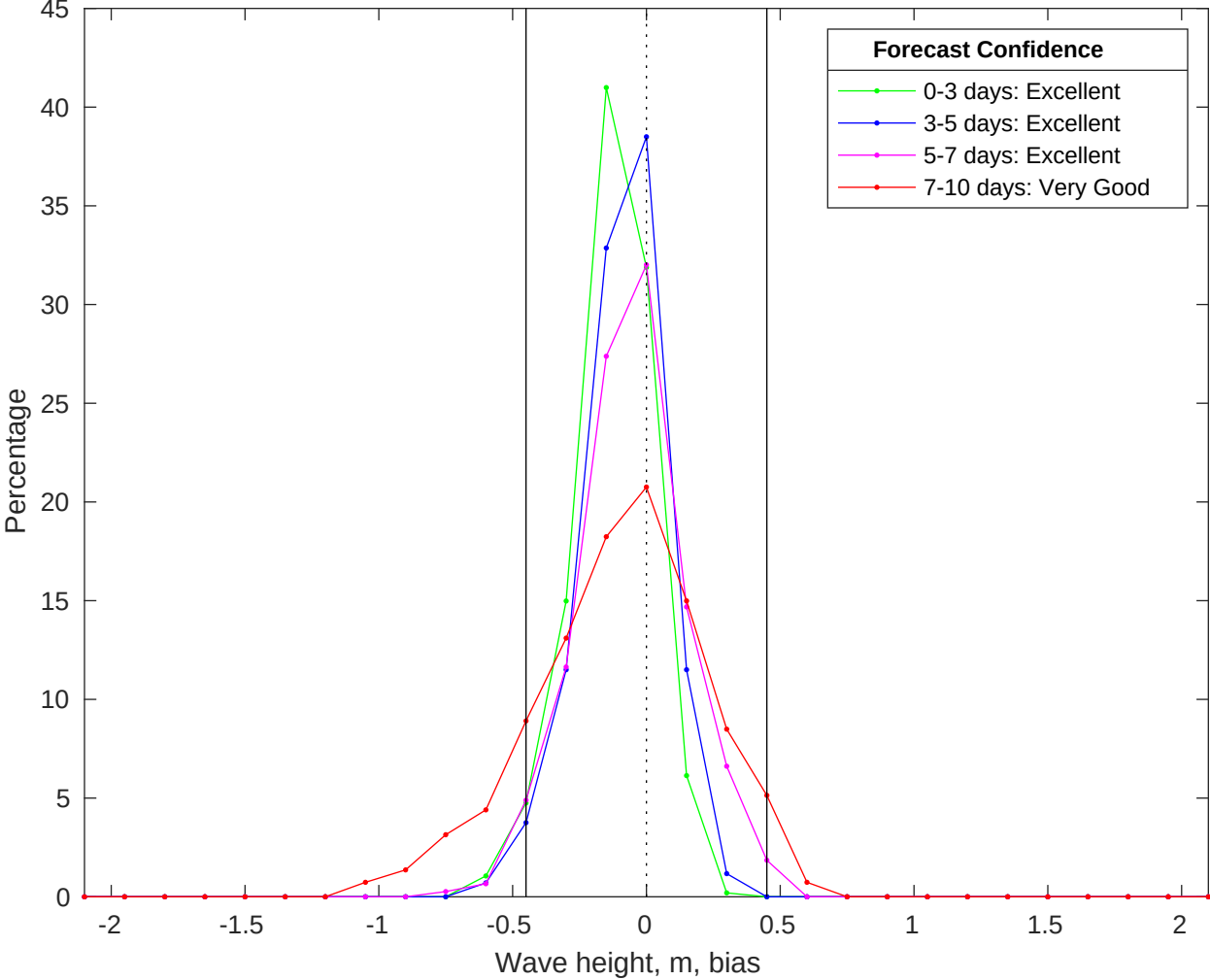
NDBC 42019 vs CMEMS Waves Bias Histogram: 02-Jun-2025
