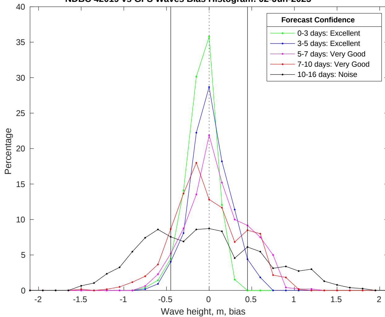
NDBC 42019 vs GFS Waves Bias Histogram: 02-Jun-2025
