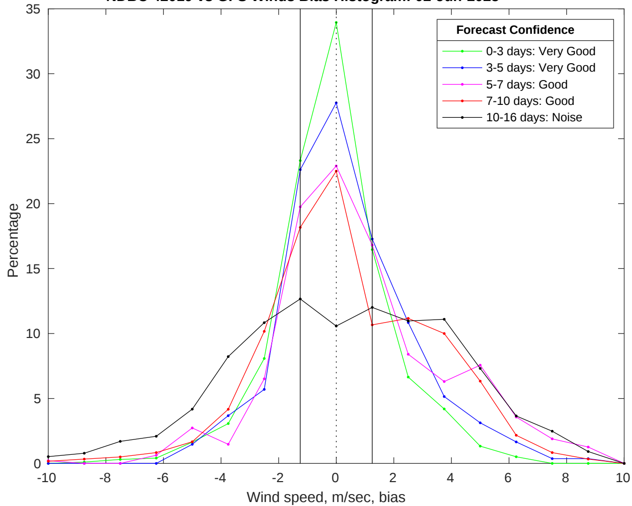
NDBC 42019 vs GFS Winds Bias Histogram: 02-Jun-2025
