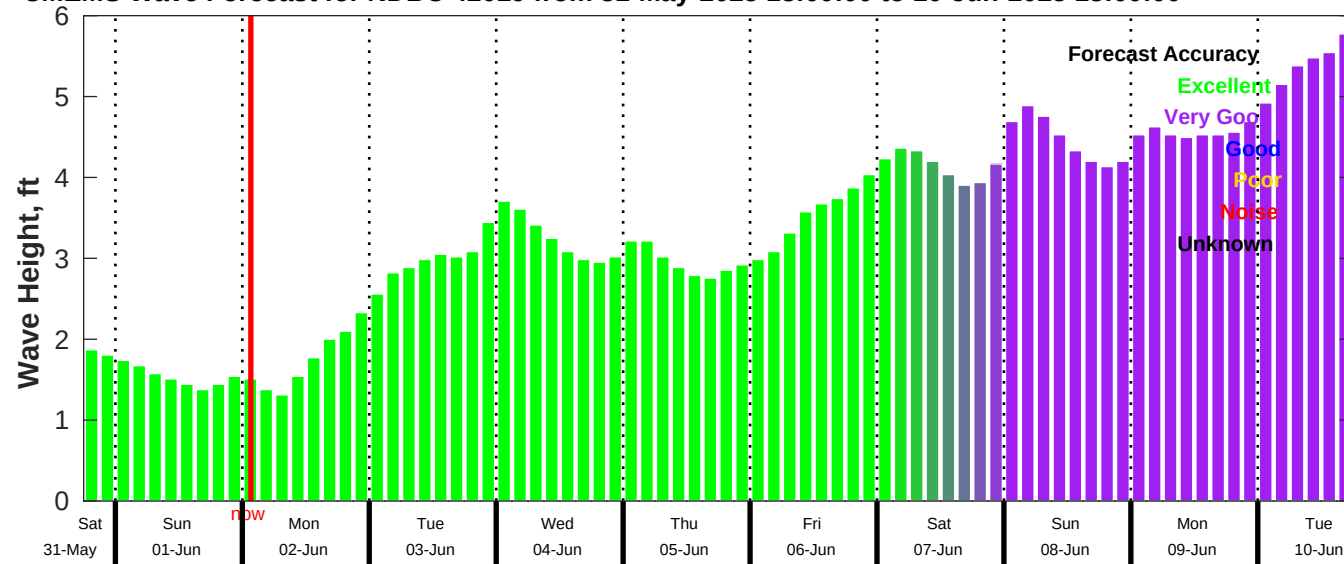
CMEMS Wave Forecast for NDBC 42019 from 31-May-2025 18:00:00 to 10-Jun-2025 18:00:00
