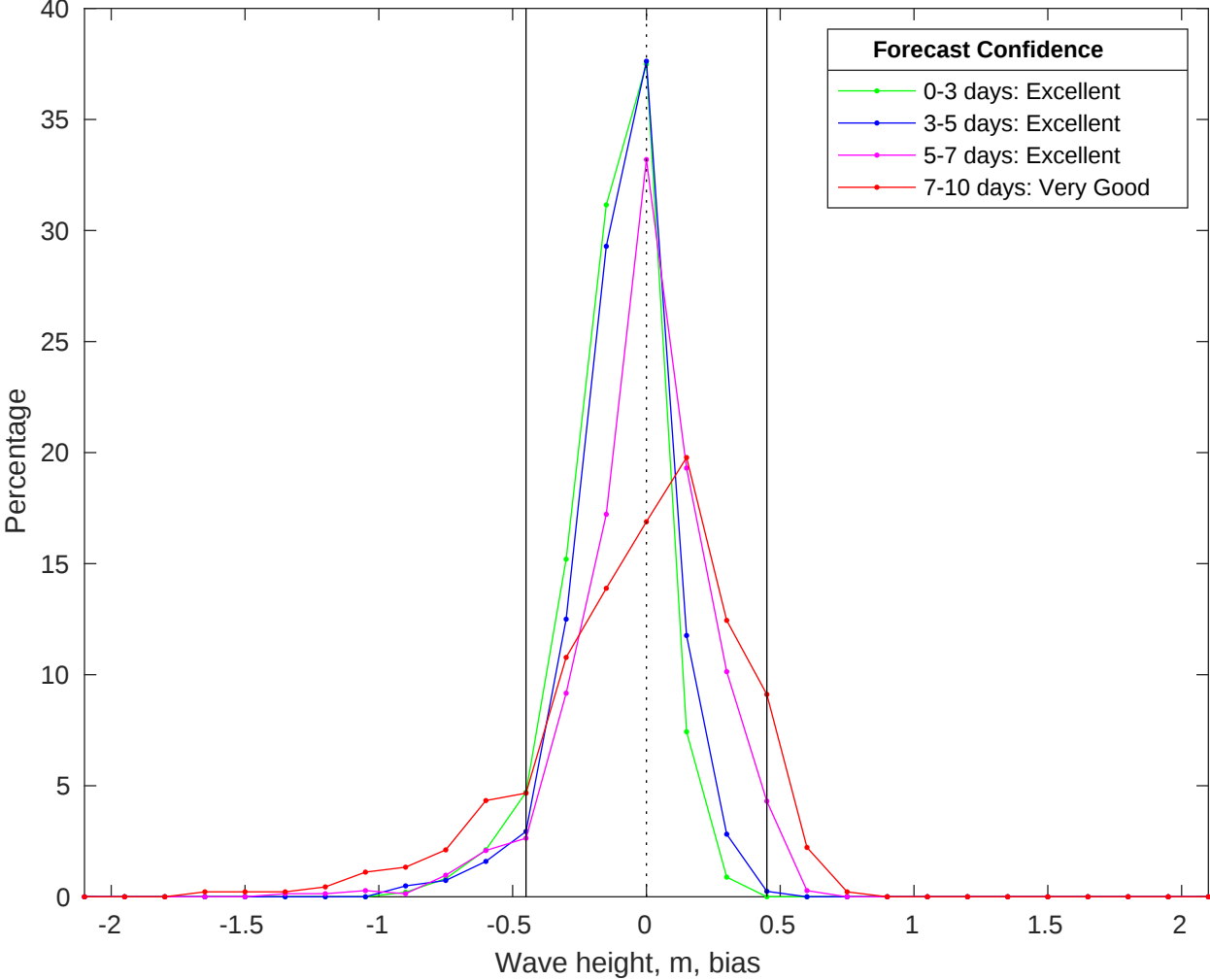
NDBC 42020 vs CMEMS Waves Bias Histogram: 01-Jun-2025
