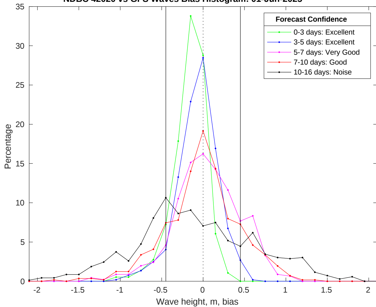
NDBC 42020 vs GFS Waves Bias Histogram: 01-Jun-2025
