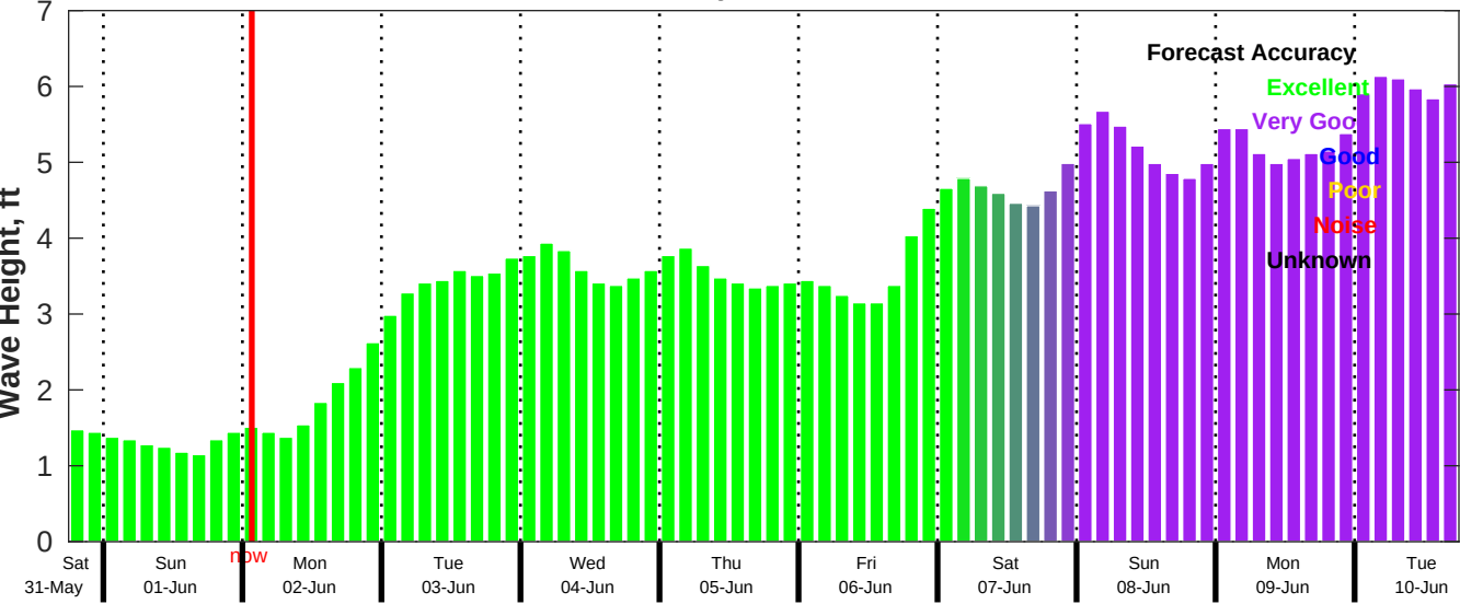
CMEMS Wave Forecast for NDBC 42020 from 31-May-2025 18:00:00 to 10-Jun-2025 18:00:00
