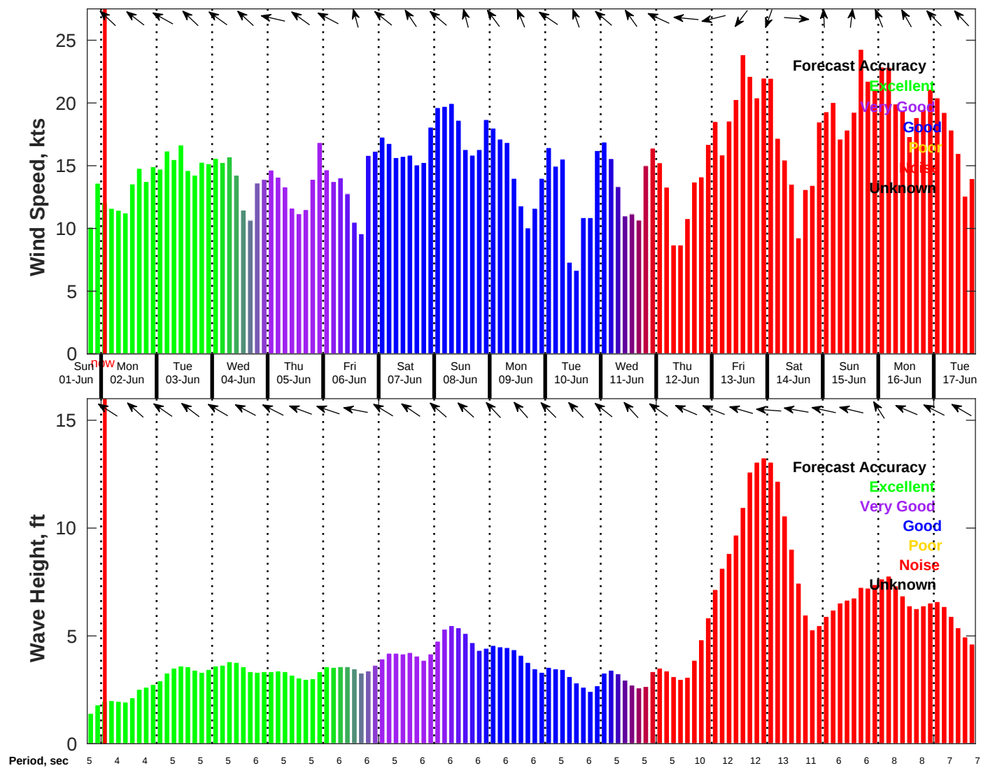
Wind & Wave Forecast for NDBC 42020 from 01-Jun-2025 18:00:00 to 17-Jun-2025 18:00:00
