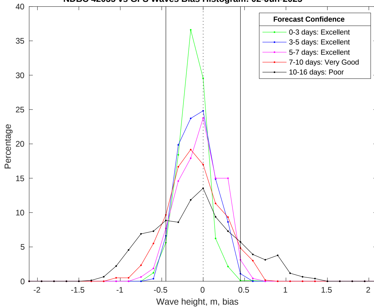
NDBC 42035 vs GFS Waves Bias Histogram: 02-Jun-2025
