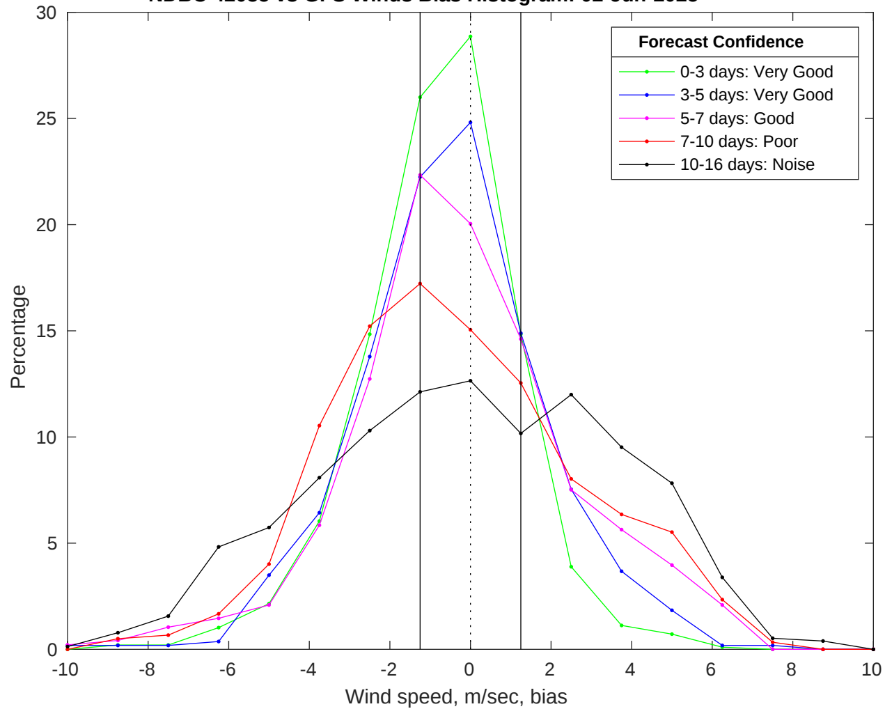
NDBC 42035 vs GFS Winds Bias Histogram: 02-Jun-2025
