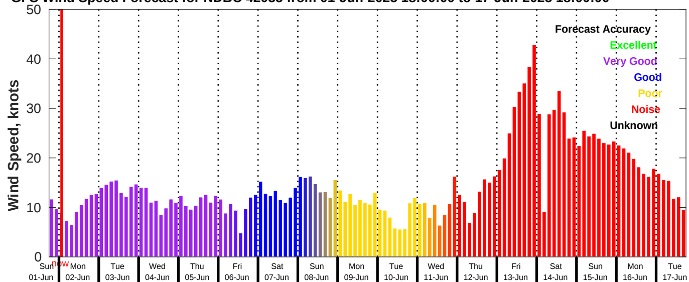
GFS Wind Speed Forecast for NDBC 42035 from 01-Jun-2025 18:00:00 to 17-Jun-2025 18:00:00
