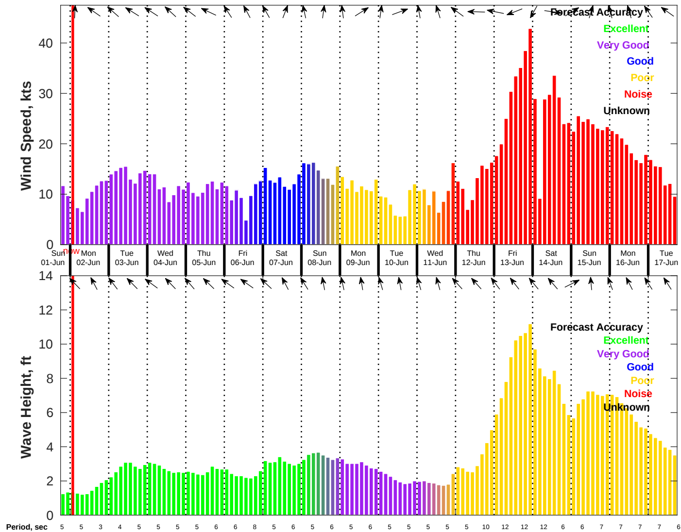
Wind & Wave Forecast for NDBC 42035 from 01-Jun-2025 18:00:00 to 17-Jun-2025 18:00:00
