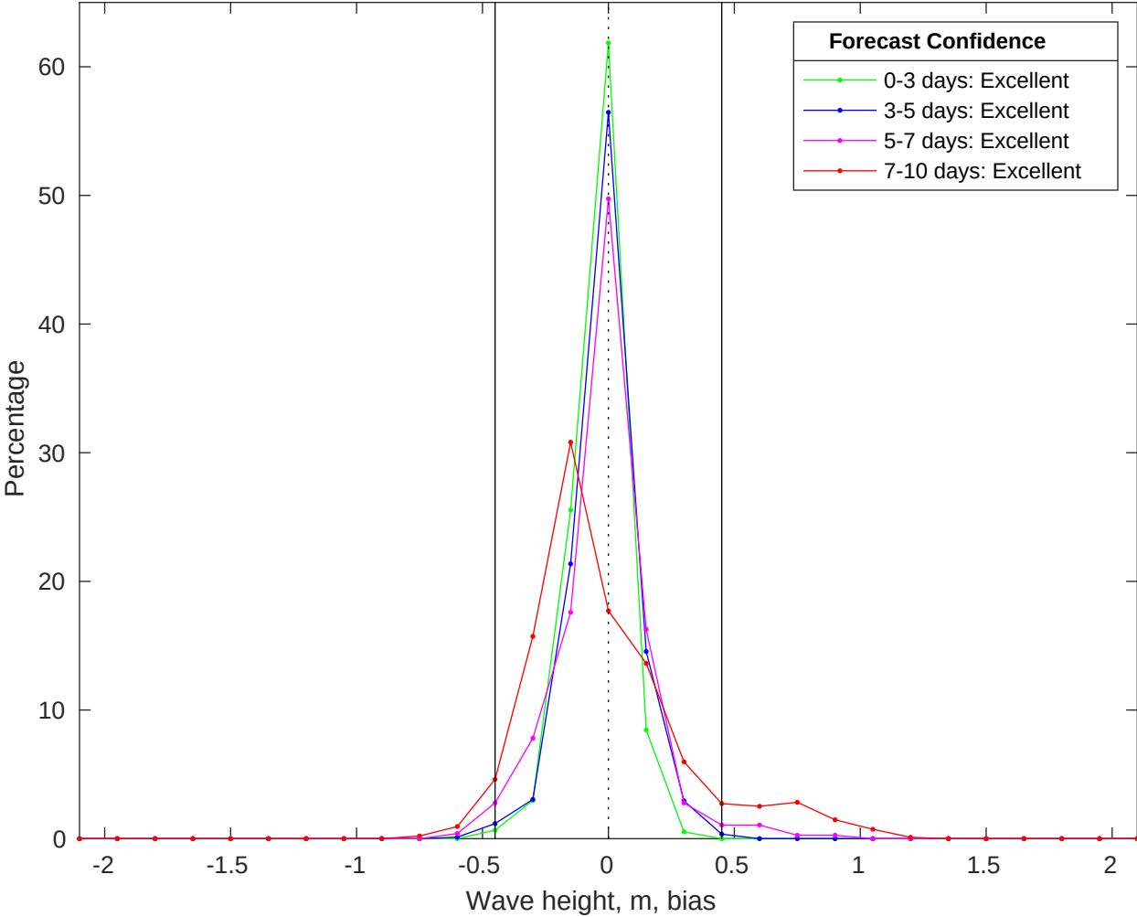
NDBC 42036 vs CMEMS Waves Bias Histogram: 02-Jun-2025
