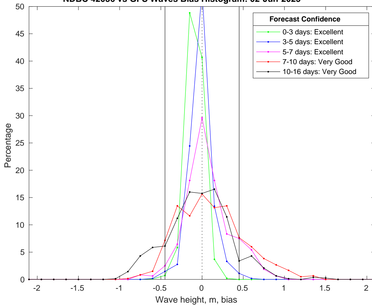
NDBC 42036 vs GFS Waves Bias Histogram: 02-Jun-2025
