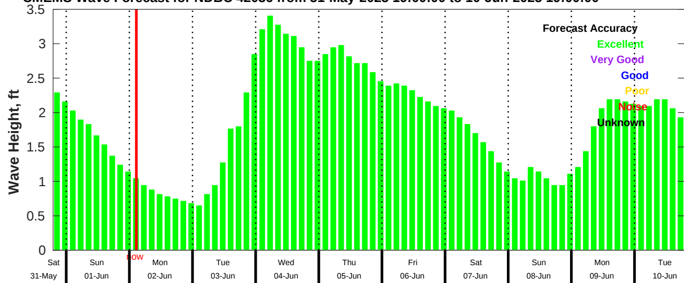
CMEMS Wave Forecast for NDBC 42036 from 31-May-2025 19:00:00 to 10-Jun-2025 19:00:00
