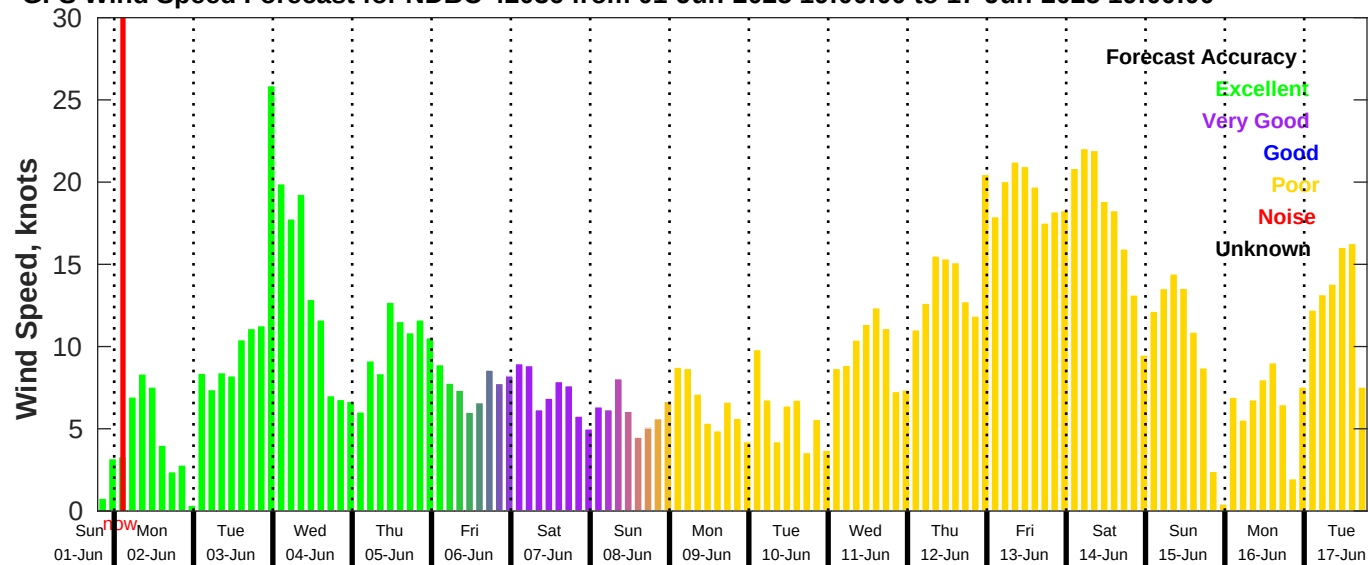
GFS Wind Speed Forecast for NDBC 42036 from 01-Jun-2025 19:00:00 to 17-Jun-2025 19:00:00
