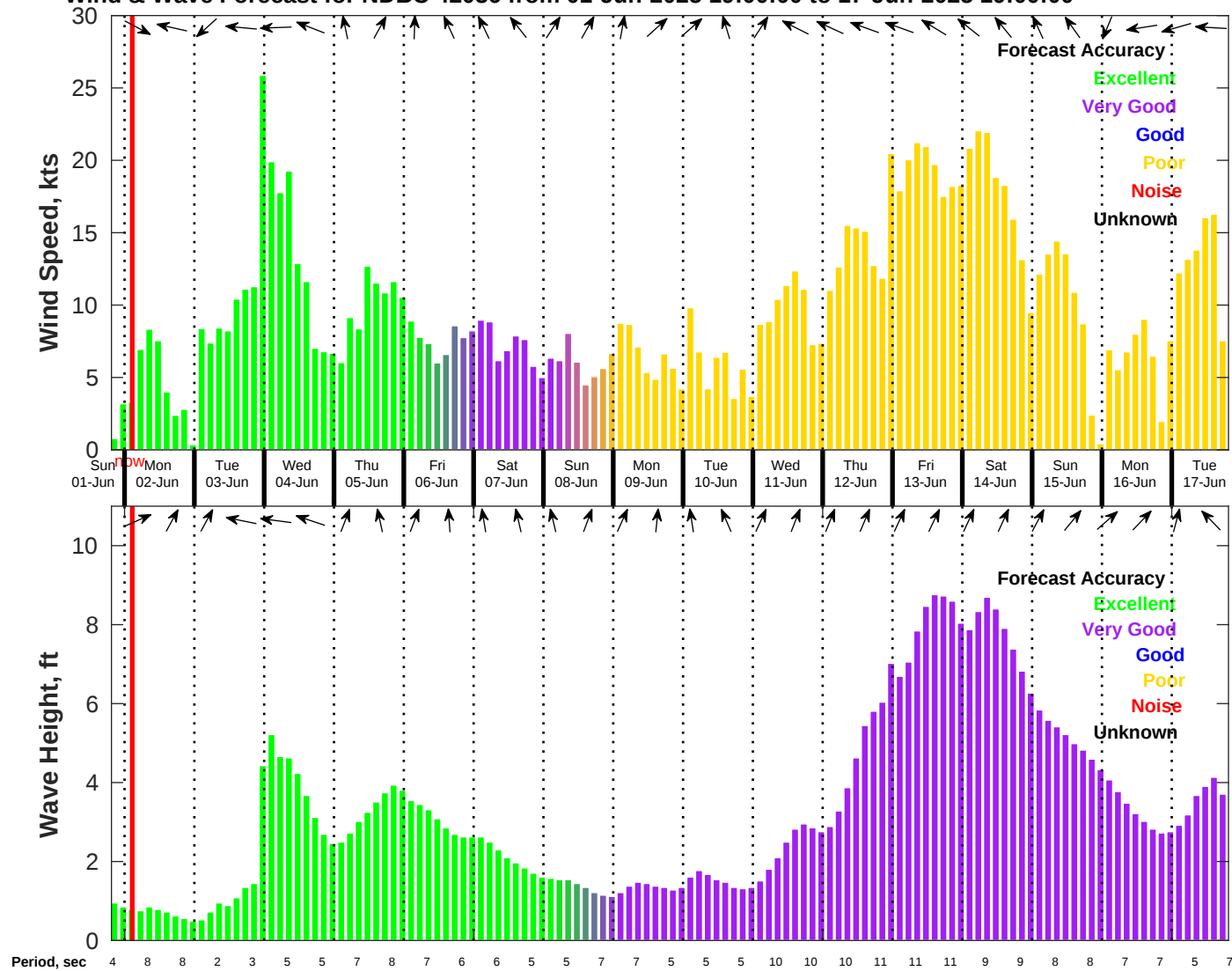
Wind & Wave Forecast for NDBC 42036 from 01-Jun-2025 19:00:00 to 17-Jun-2025 19:00:00
