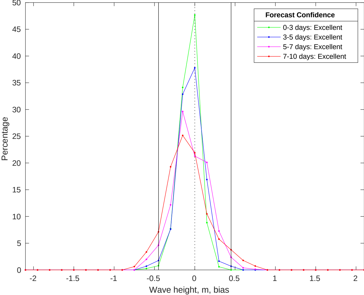
NDBC 42040 vs CMEMS Waves Bias Histogram: 02-Jun-2025
