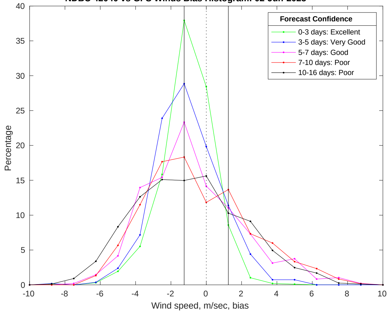
NDBC 42040 vs GFS Winds Bias Histogram: 02-Jun-2025
