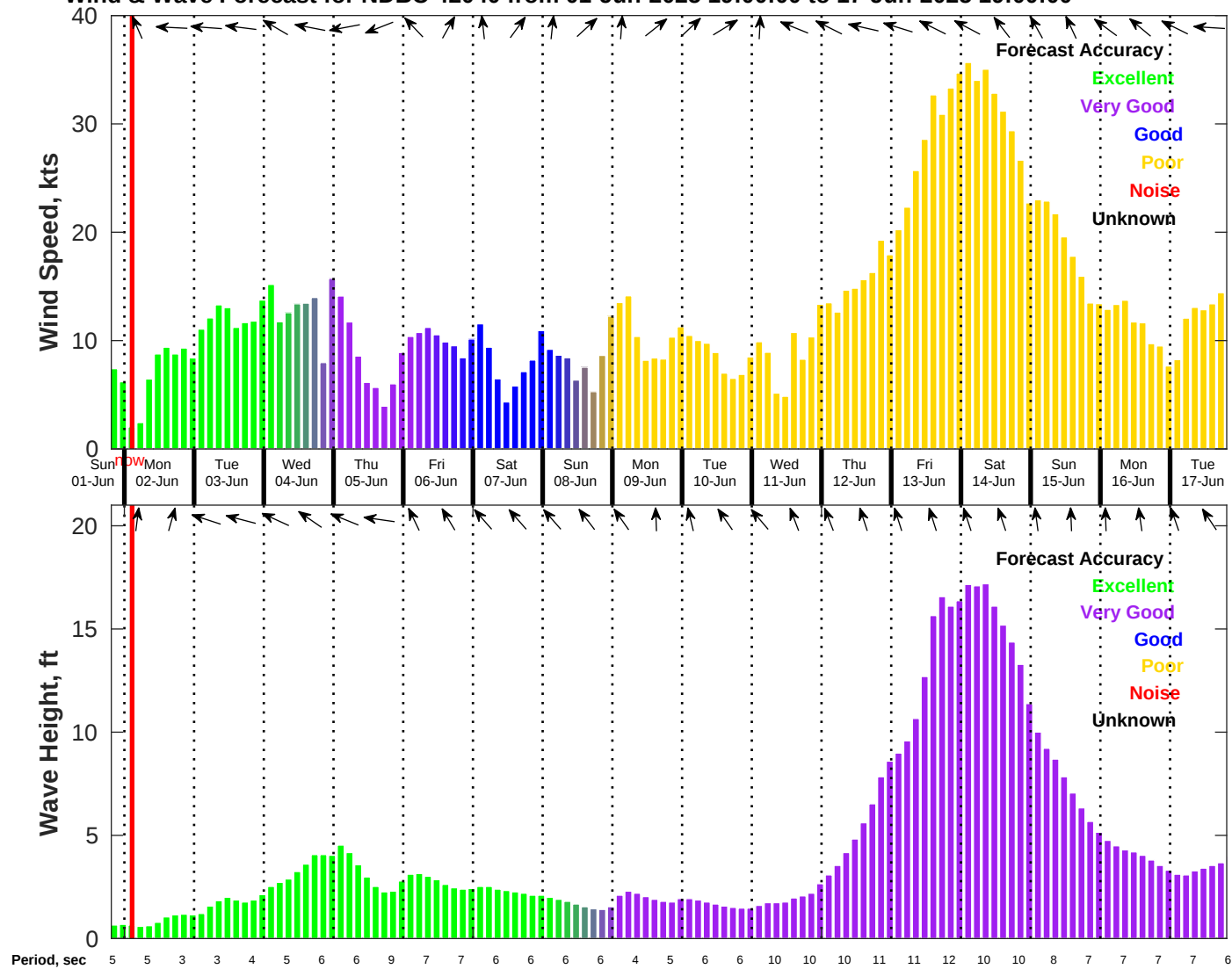
Wind & Wave Forecast for NDBC 42040 from 01-Jun-2025 19:00:00 to 17-Jun-2025 19:00:00
