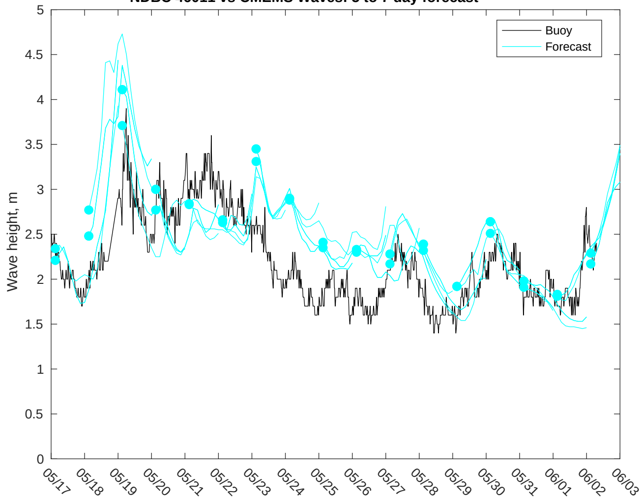
NDBC 46011 vs CMEMS Waves: 5 to 7 day forecast
