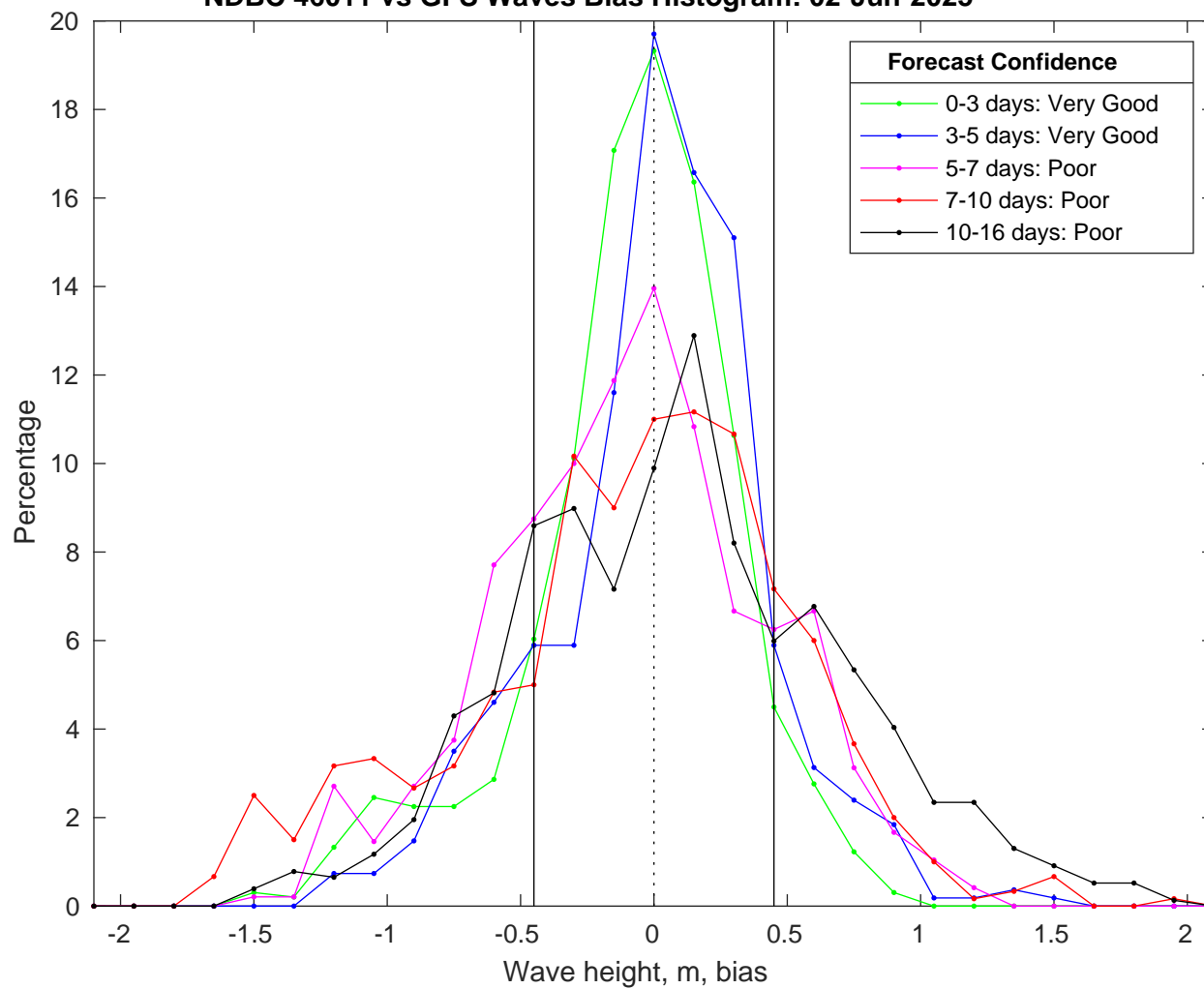
NDBC 46011 vs GFS Waves Bias Histogram: 02-Jun-2025
