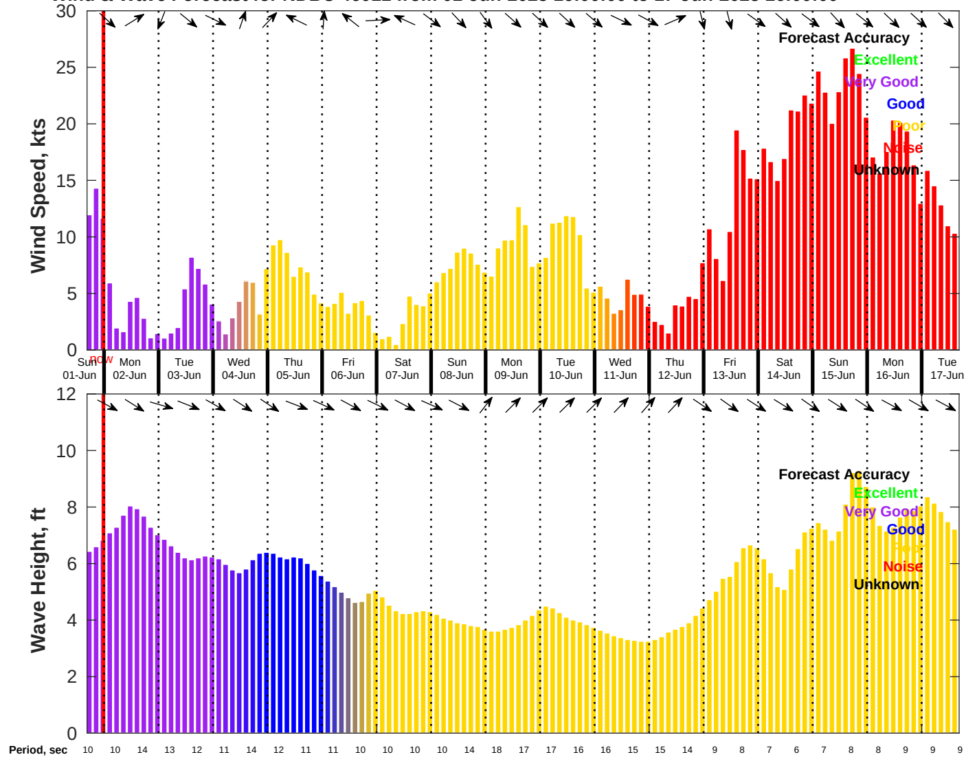
Wind & Wave Forecast for NDBC 46011 from 01-Jun-2025 16:00:00 to 17-Jun-2025 16:00:00
