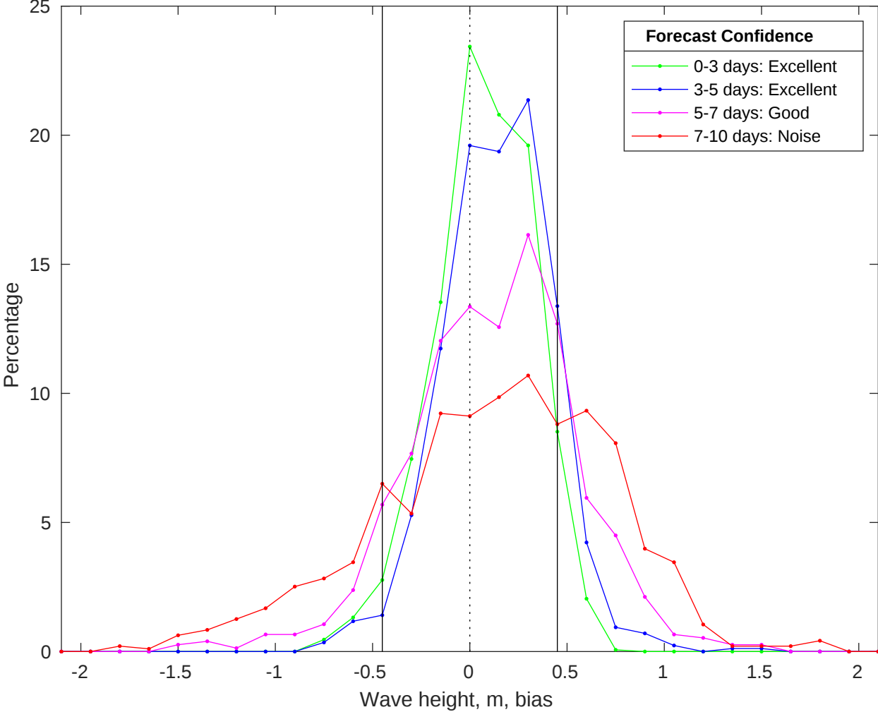
NDBC 46028 vs CMEMS Waves Bias Histogram: 02-Jun-2025
